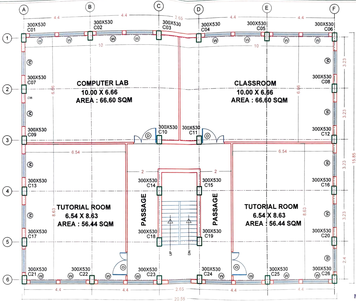
SECOND FLOOR ( MULTI-PURPOSE HALL BUILDING )
